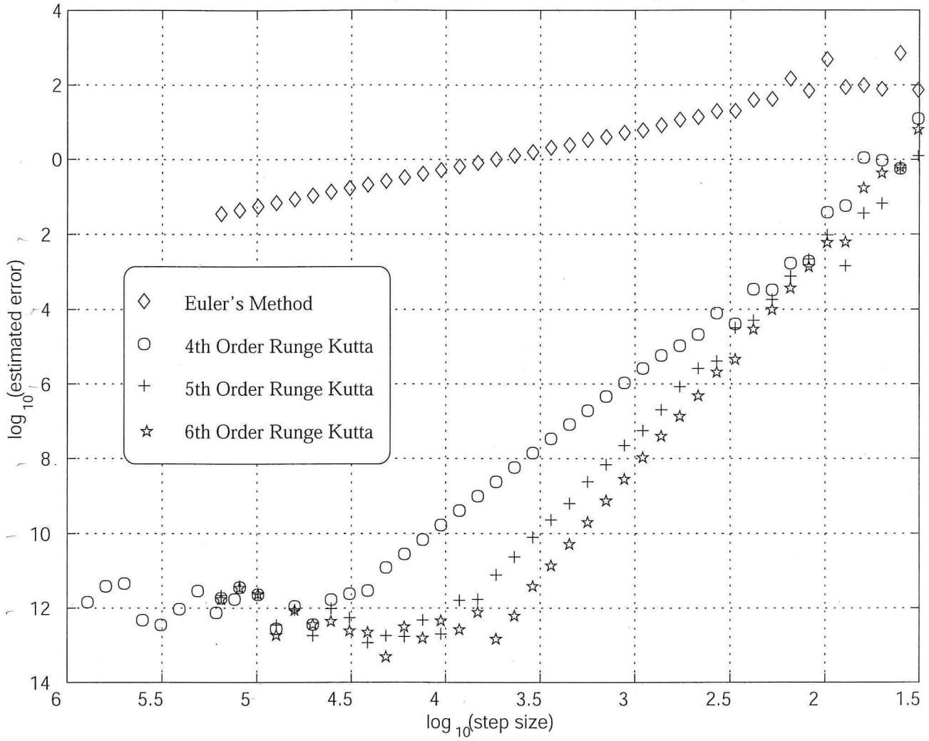
Numerical Accuracy for collisionsless walker taking a 1/2 step
